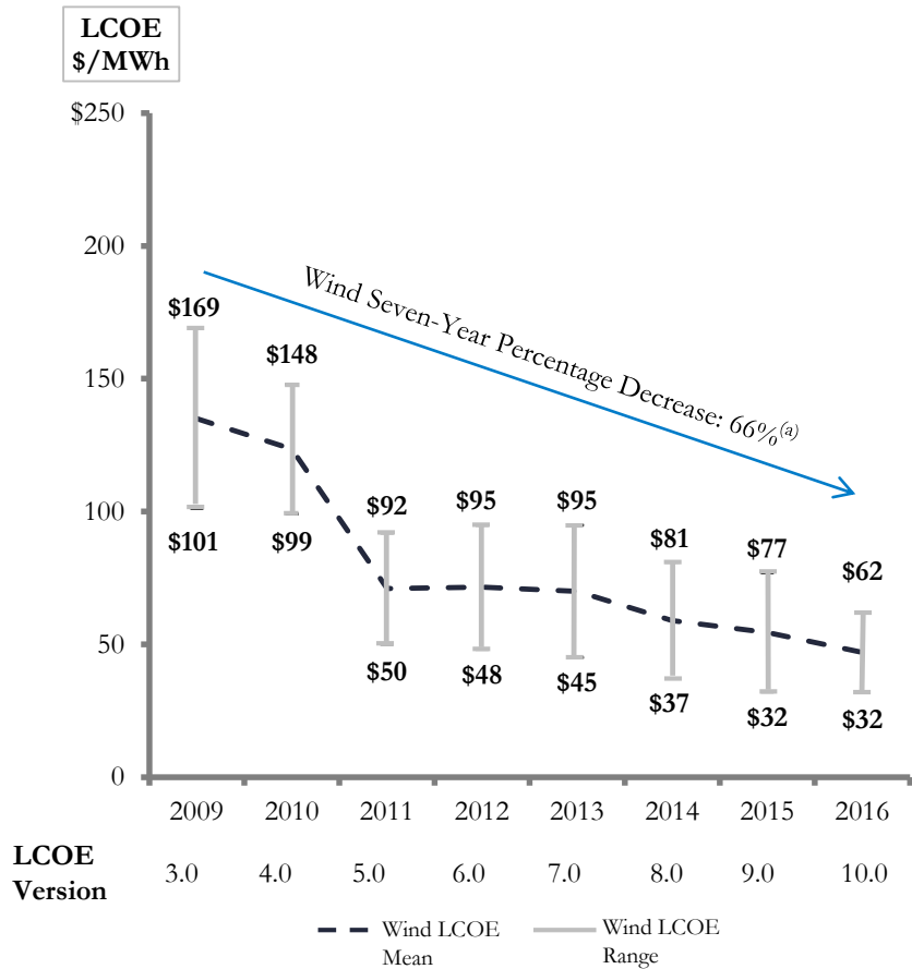
WIND LCOE
